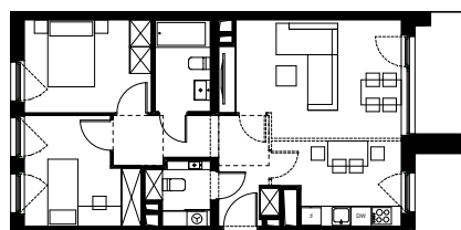
APARTMENT M3_L AREA: 64,38 sqm
