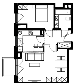
APARTMENT M2_L AREA: 49,58 sqm
